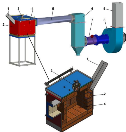
Fig. 7. Scheme of the experimental facility for BMW plasma gasification: 1 – an inlet for loading briquetted BMW into the reactor, 2 – a plasma reactor, 3 – an electric-arc direct current plasma torch, 4 – a BMW gasification zone, 5 – an off-gas cooling unit, 6 – a gas-cleaning unit with a bag filter, 7 – an exhaust gas tube with a system for gas sampling and temperature measurement, 8 – an exhaust fan, 9 – an exhaust tube. In the experiments, the BT consumption G_{BT} varied within 5.4–10.8 kg/h. The amount of the plasma-forming
