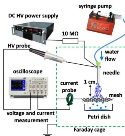
Fig. 1. Experimental set-up of air transient spark with water electrospray.
